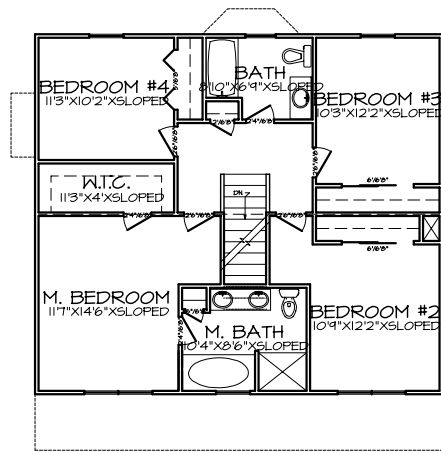
1 SECOND FLOOR PLAN A-5
