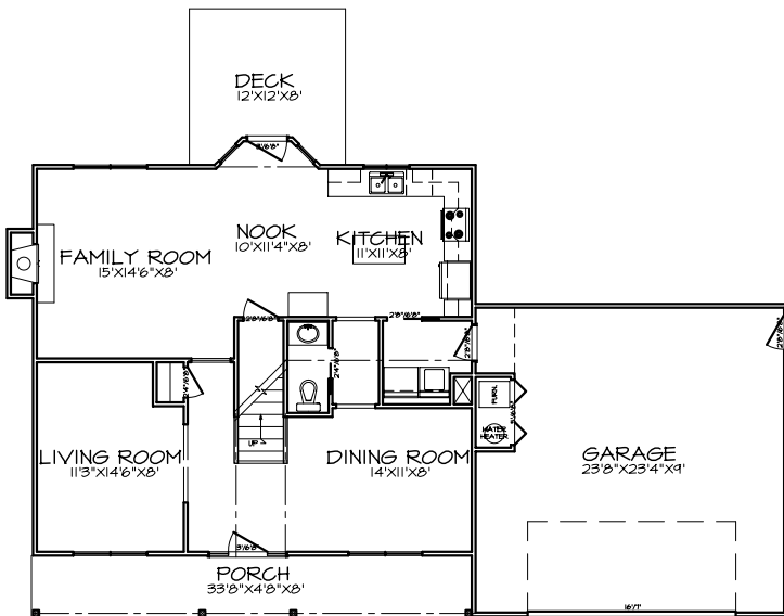
1 FIRST FLOOR PLAN A-4
