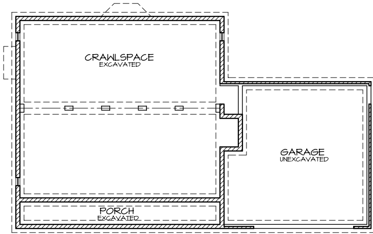
1 FOUNDATION PLAN A-3
